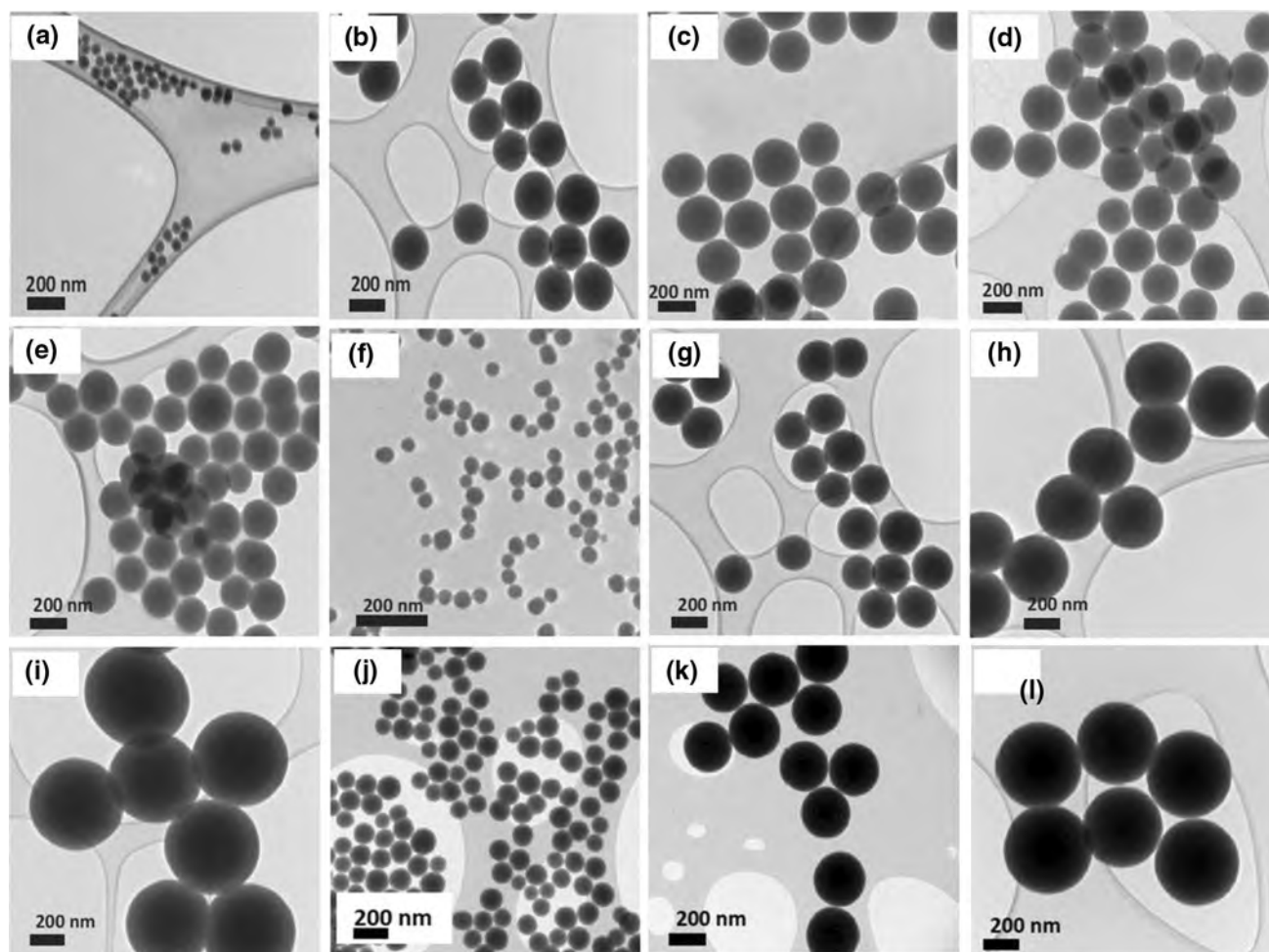
Fig. 7 Transmission electron microscopy (TEM) of silica particles. a–d fixed concentration of tetraethylorthosilicate (TEOS), ammonia solution ( \text{NH}_4\text{OH} ) and varied amounts of water. Fixed concentration of TEOS and water, and varied concentration of \text{NH}_4\text{OH} f 0.11 M, g 0.28 M, h 0.57 M, i 1.13 M, j 0.17 M, k 0.40 M, l 0.85 M, reprinted
